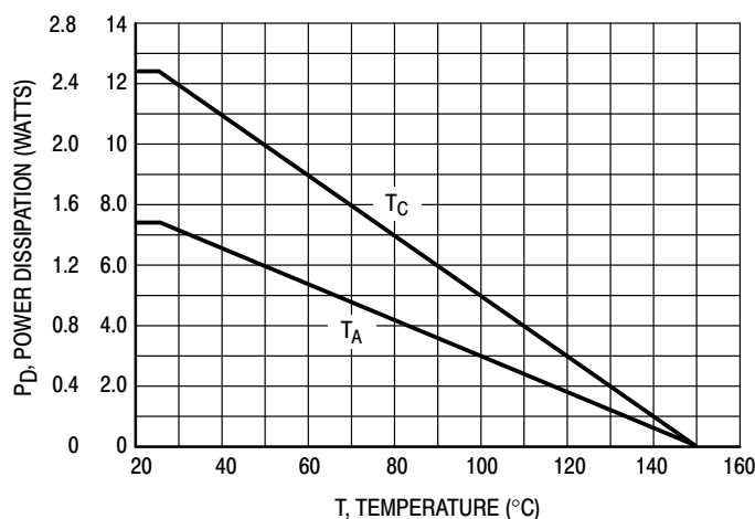
Figure 1. Power Derating
